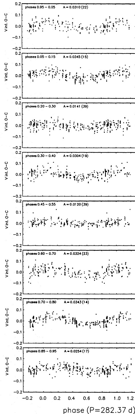
Fig. 13. The 282.370-d phase curves shown for various subsets of V -intensity residuals selected in 0 P .1 wide bins for different orbital phases of \beta Lyr. It illustrates how the amplitude, phase and scatter for the 282.37-d period vary with the orbital phase. The semi-amplitude A and its rms error are given for each orbital-phase bin shown
