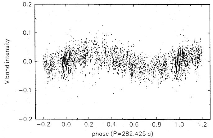
Fig. 12. All V-band intensity residuals from the orbital light curve of \beta Lyr plotted vs. phase of the best-fit period of 282^d425 . An arbitrary epoch HJD 2400000 was chosen in this and following plots as phase zero.
