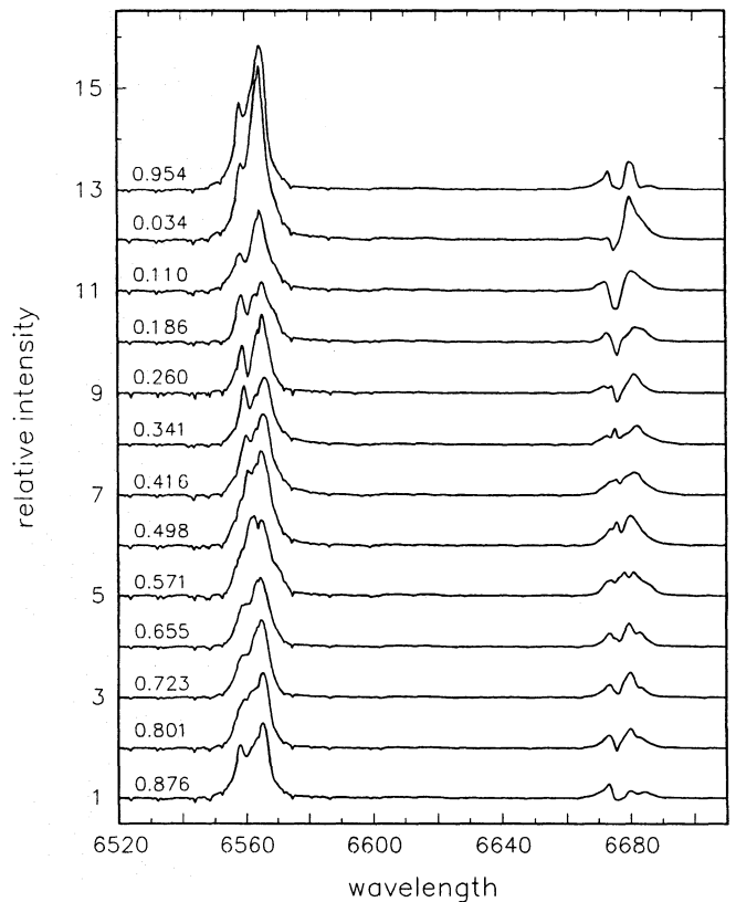
Fig. 5. Examples of the observed Reticon H\alpha and He I 6678 line profiles of \beta Lyr at various orbital phases, given for each spectrum
