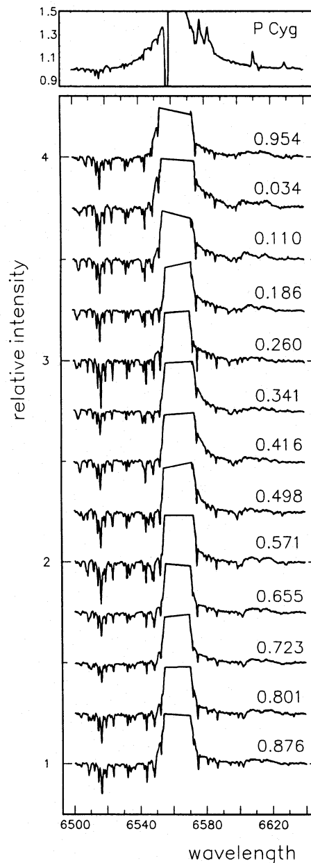
Fig. 7. Enlarged spectra in the neighbourhood of H\alpha , showing the character of the extended emission wings and also a weak broad emission feature at about 6611 \text{ \AA} . Corresponding orbital phases are given for each spectrum. Note that the upper parts of the H\alpha emission were artificially removed to increase the contrast of the bottom parts of the line profiles. For comparison, a Reticon spectrum of P Cyg is also shown
